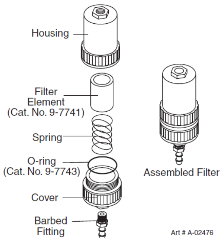
Optional Single - Stage Filter Kit
